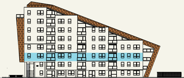
WEST ELEVATION
